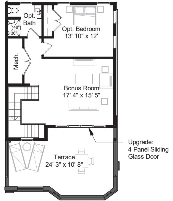
TERRACE LEVEL BEDROOM OPTION
