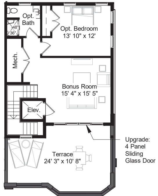
TERRACE LEVEL BEDROOM OPTION w/ ELEVATOR OPTION
