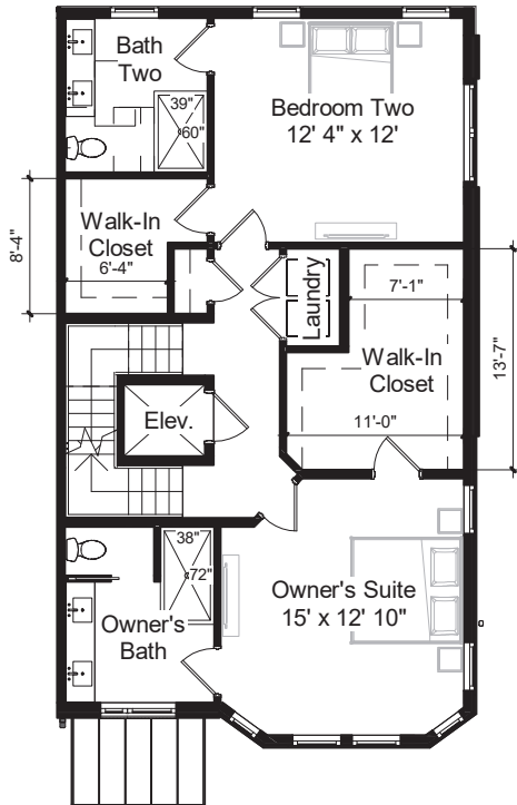
BEDROOM LEVEL TWO BEDROOM OPTION w/ ELEVATOR OPTION
