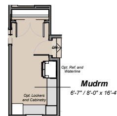
Alternative Mudroom Layout w/ Second Floor Laundry
