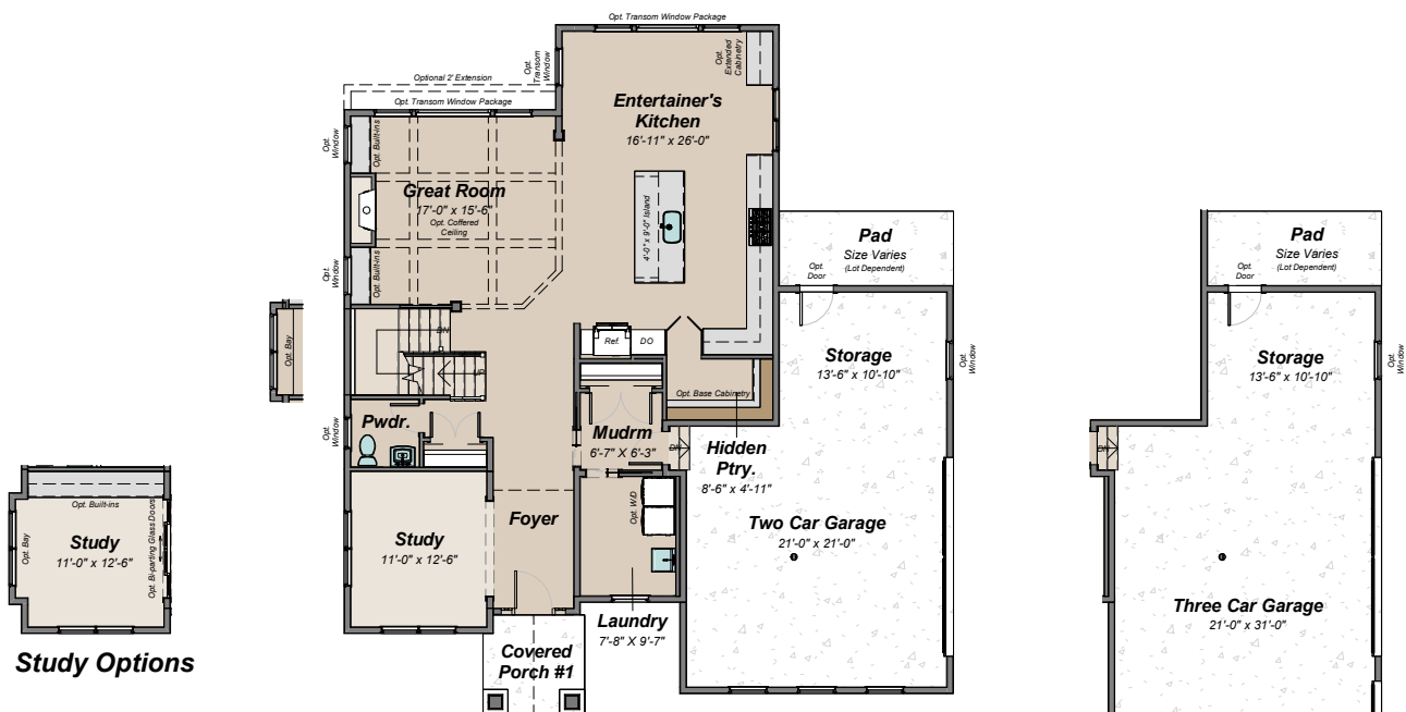
INCLUDED FIRST FLOOR Standard 10'-0" Ceilings
