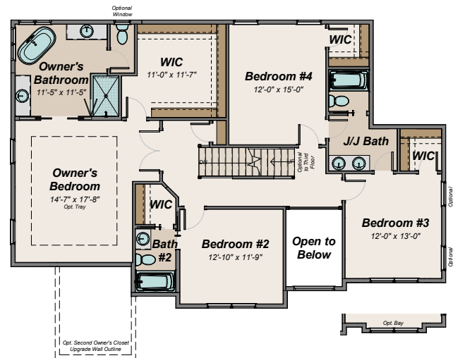
INCLUDED SECOND FLOOR
