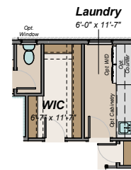
Optional Laundry (With Included Second Floor)
